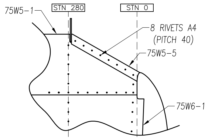
BOTTOM VIEW: RIVET LOCATIONS ON ROOT SKIN
