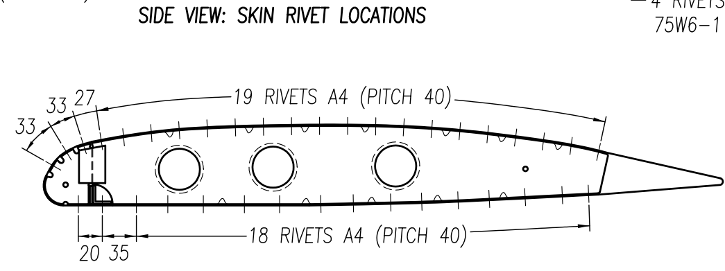
SIDE VIEW: SKIN RIVET LOCATIONS FOR ROOT RIBS
