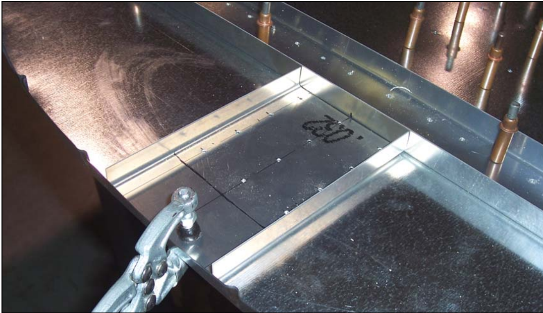
P/N: 75F9-7 Upper Firewall Channel
