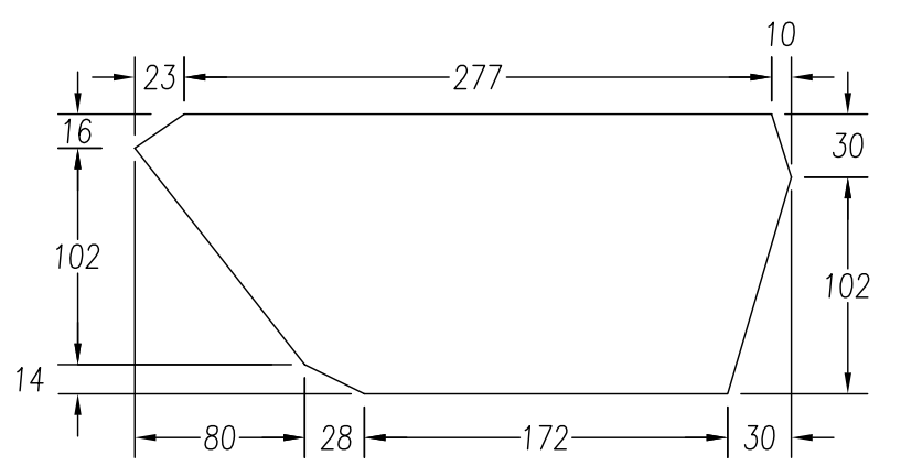
② SIDE SKIN DOUBLER t=0.032inch 6061-T6 (2 req'd) SUPPLIED PRE-DRILLED
