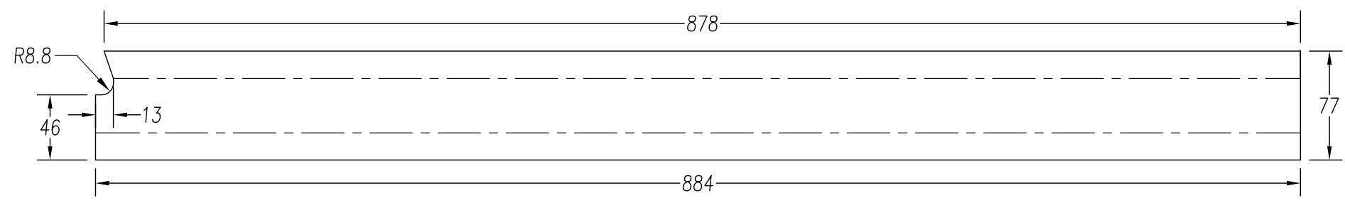
① BAGGAGE BACK CHANNEL t=0.032inch 6061-T6 (2 req'd)
