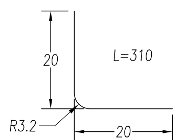
③ SIDE SKIN ANGLE t=0.032inch 6061-T6 (2 req'd)
