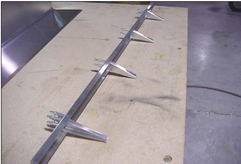
7A1-4 Flaperon Spar 7A1-3 Flaperon Rear Ribs
