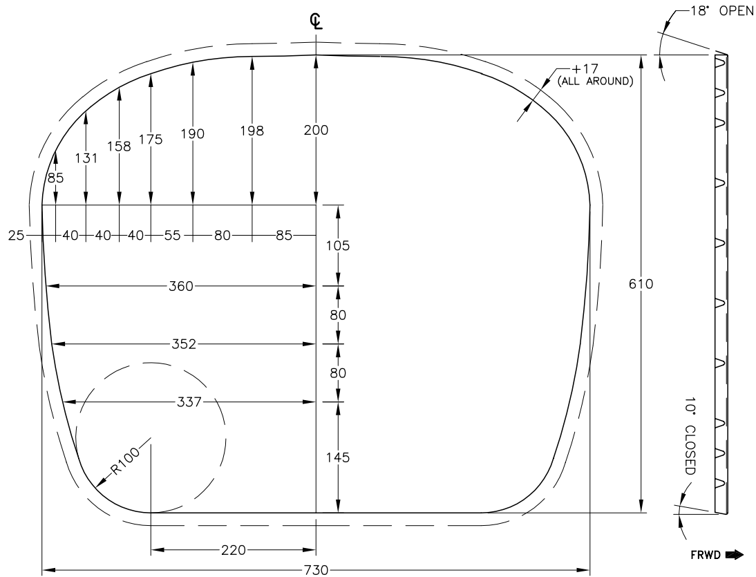
FIREWALL t=.018" GALVANIZED STEEL (1 REQ'D)
