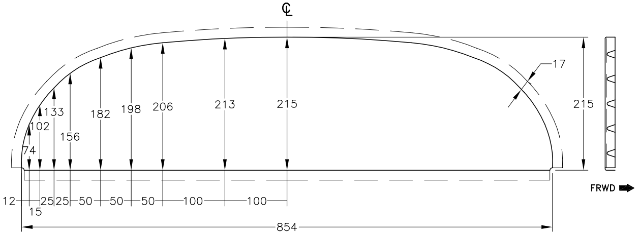
INSTRUMENT PANEL BULKHEAD t=.025" (1 REQ'D)
