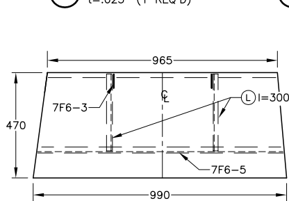
4 SEAT BACK t=.016" (1 REQ'D)
