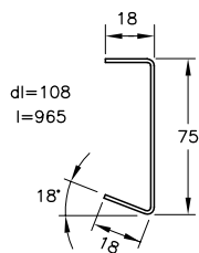
1 BOTTOM CHANNEL t=.025" (1 REQ'D)
