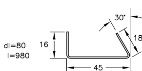
5 SEAT BACK CHANNEL t=.025" (1 REQ'D)
