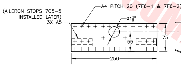
2 REAR TORQUE TUBE BEARING t=.063" (1 REQ'D)
